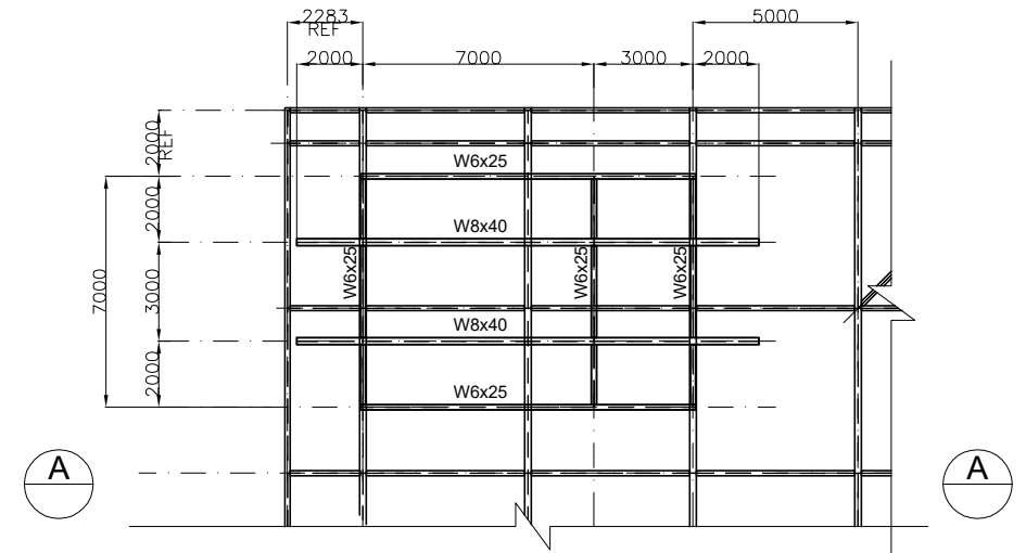
FRAMING PLAN @ EL. + 6000 SCALE 1:250
