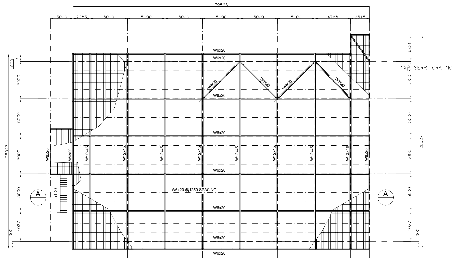
BUBOUWE PLATFORM FRAMING PLAN @ EL. + 3000 SCALE 1:250
